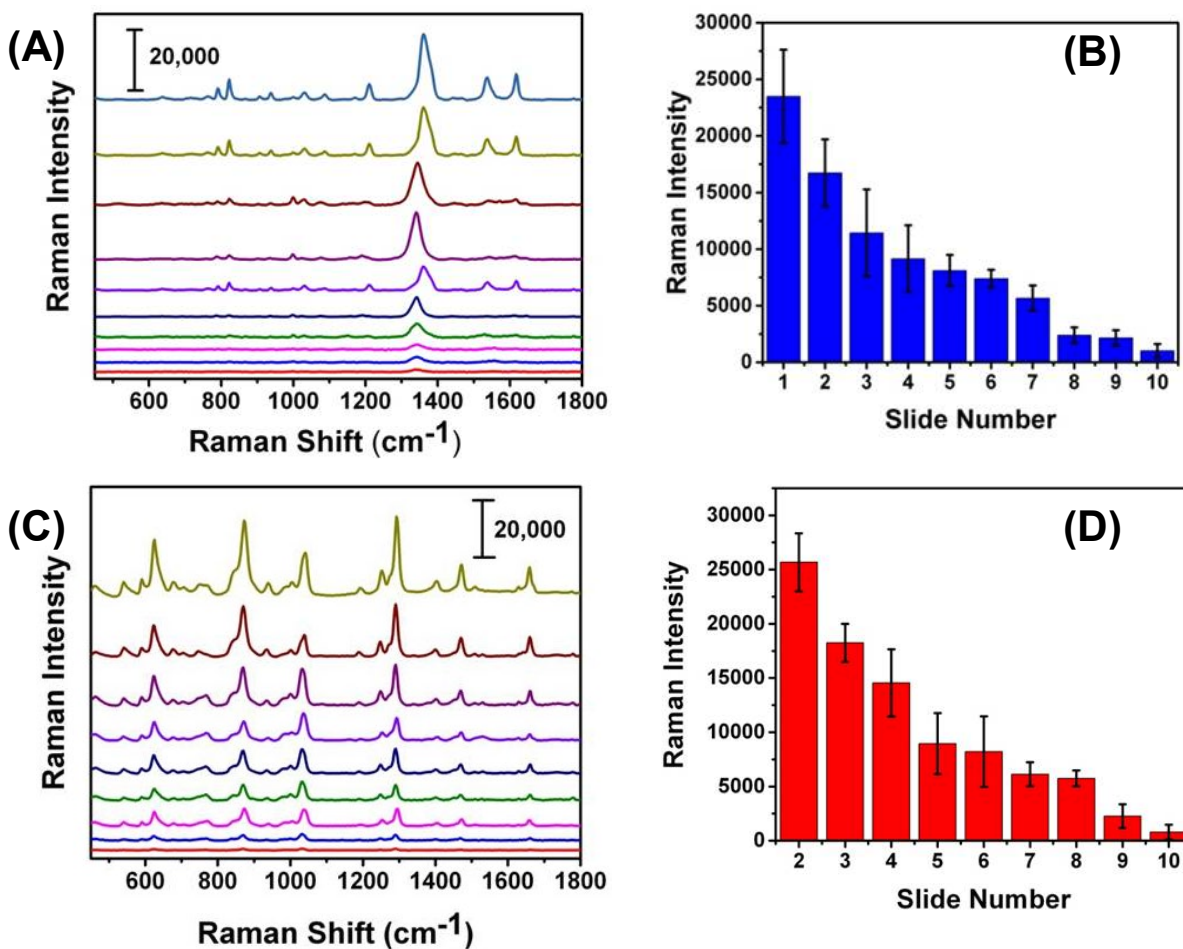
Fig. 7. SERS nanosensor spectra of (A) TNT and (C) PETN collected by transferring fingerprint explosive residue from glass to SERS nanosensors. The top and bottom spectra are number 1 and 10 glass slides in which explosives powder was transferred from 1 to 2 to higher number slides through subsequent thumb pressing with the thumb exposed only once and depositing a decreasing amount of residue on each slide. The plot of SERS intensity (B) TNT (1380 \text{cm}^{-1} ) and (D) PETN (1290 \text{cm}^{-1} ) as function of slide number. Scale bars in (A) and (C) represent counts per second.
