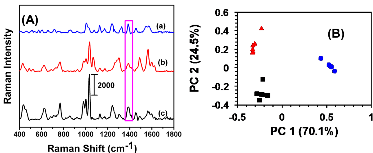
Fig. 3. (A) Representative SERS spectra acquired using the nanosensor from 100 fM: (a) TNT, (b) TNB, and (c) DNT at 1380 \text{cm}^{-1} (purple box). Scale bar represents counts per second. (B) Plot of PCA scores for SERS at 100 fM concentration of TNT (blue spheres), TNB (red triangles), and DNT (black square). DA classified 100% of spectra correctly. Here n=18 , DA prediction 100%.
