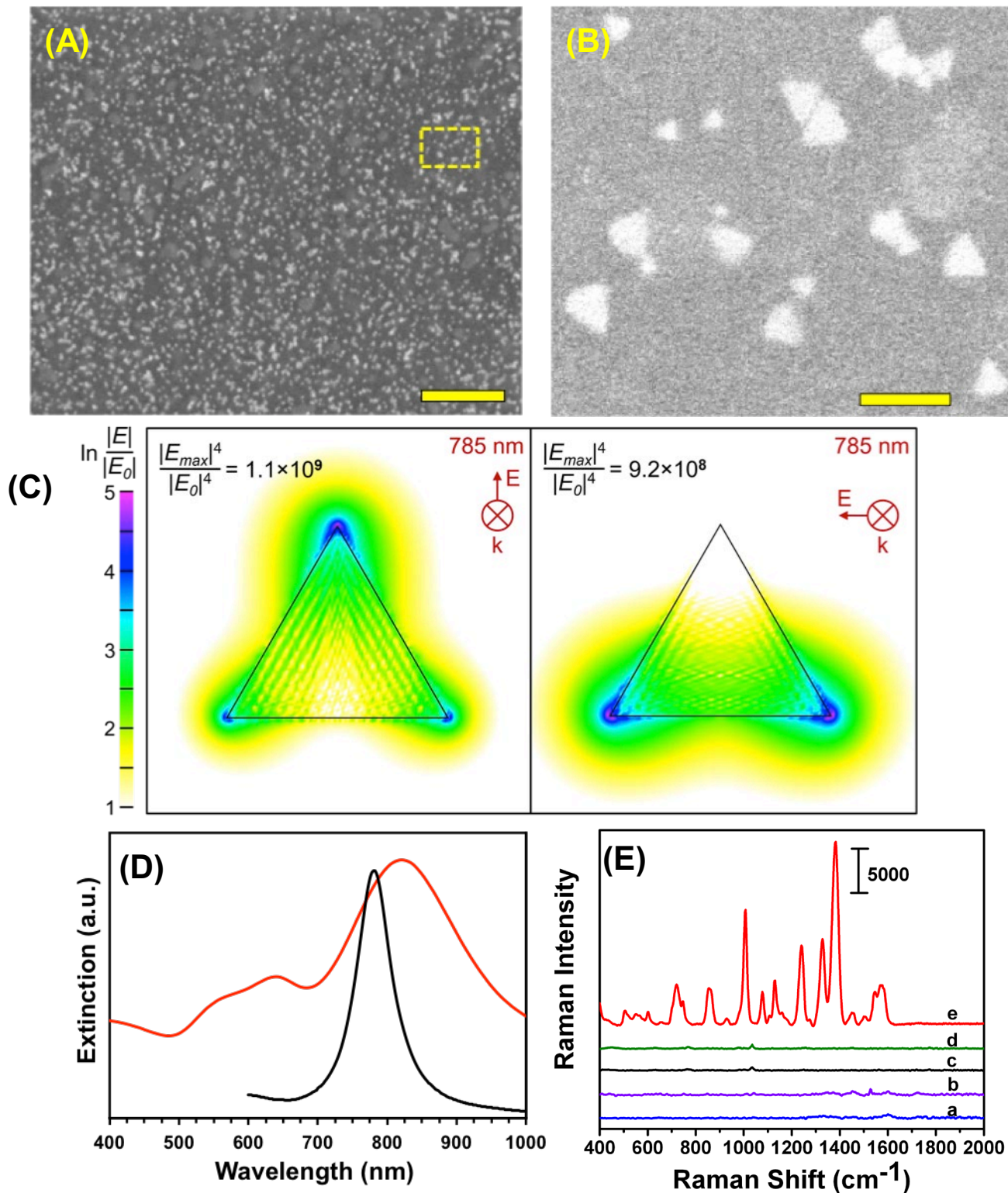
Fig. 2. (A) Low magnification SEM image of our SERS nanosensor (1.0 \mu\text{m} scale bar). (B) High magnification SEM image of the expanded region of the nanosensor shown in dotted box in (A). Scale bar is 100 nm. (C) DDA simulated EM-field for a TOA-coated Au TNP (42 nm edge length,
